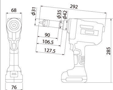
When the M6(included in N1B1) is mounted (mm)
